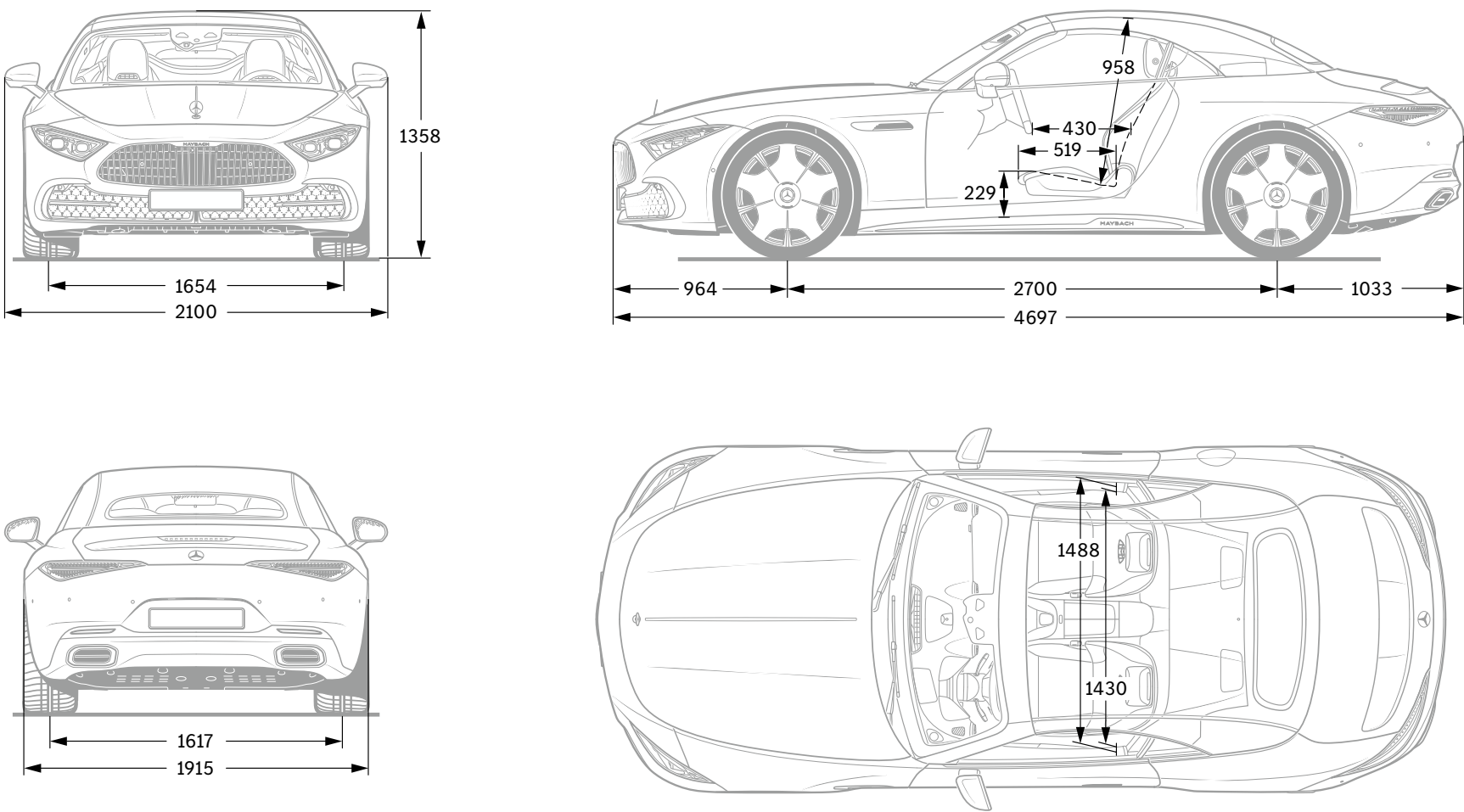
All figures in millimetres. The dimensions shown are mean values. They are valid for vehicles with standard equipment and in unladen condition.
