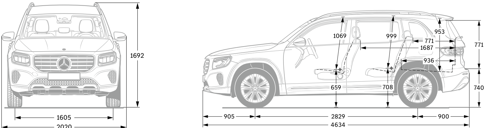
Vehicle length not including number plate adapter (4 mm).
