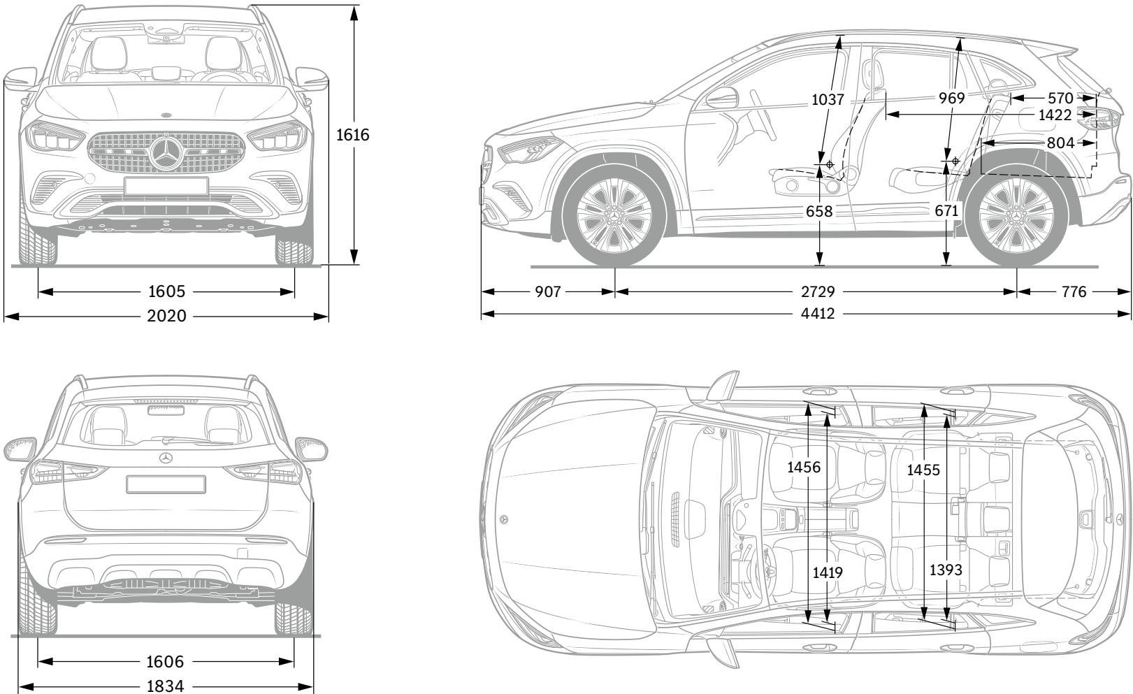
All figures in millimetres. The dimensions shown are mean values. They are valid for vehicles with standard equipment and in unladen condition.
